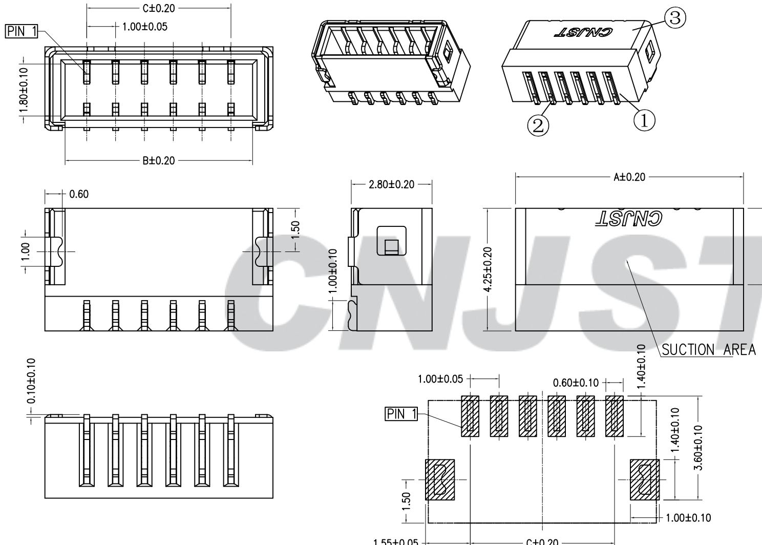
SUGGESTED PCB LAYOUT (COMPONENT SIDE)
