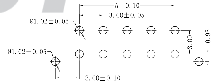
SUGGESTED PCB LAYOUT (COMPONENT SIDE)
