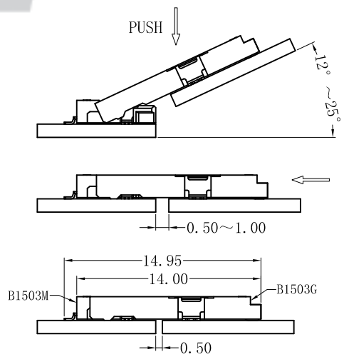
MATING VIEW SCALE 1:2
