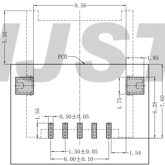
SUGGESTED PCB LAYOUT (COMPONENT SIDE)
